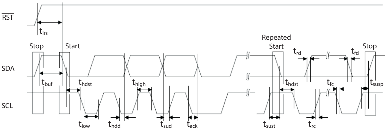
Figure 4. I 2 C Timing
