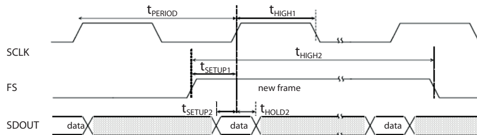
Figure 3. TDM Timing
