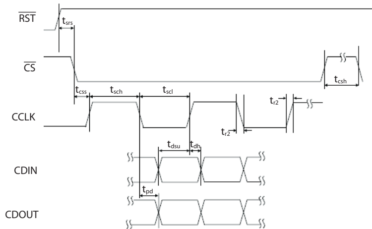
Figure 5. SPI Timing
