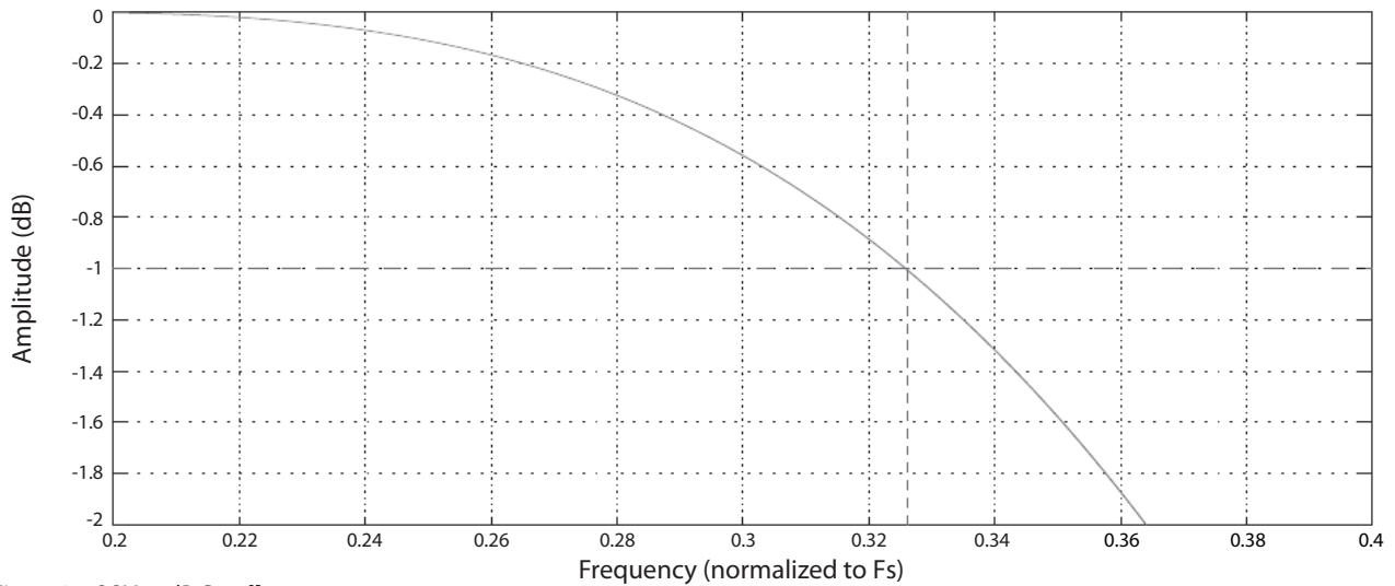
Figure 26. QSM -1 dB Cutoff
