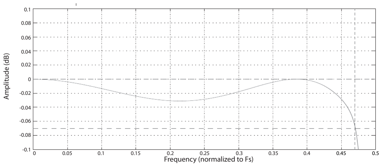
Figure 18. SSM Pass band
