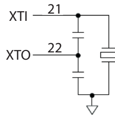
Figure 6. Crystal Oscillator Topology
